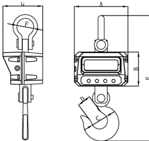
Dimensions and Capacity ( All measurements are in mm )
